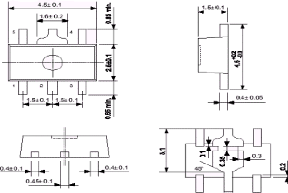
SOT89-5
