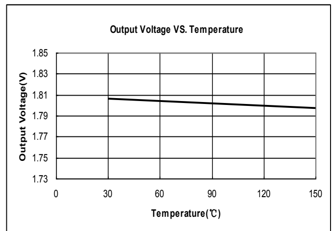
ME6118A18B3G ( V_{IN}=V_{OUT}+1.2V , I_{OUT}=10mA )
