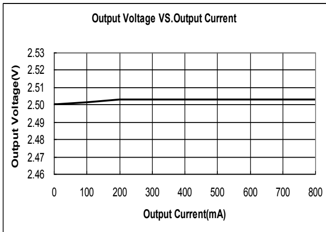
ME6118A25B3G ( V_{IN}=V_{OUT}+1.2V )
