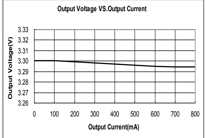
ME6118A33B3G ( V_{IN}=V_{OUT}+1.2V )
