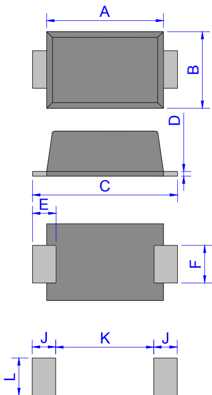
SOD-123FL
