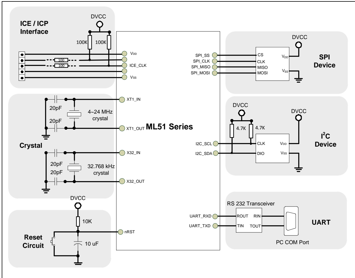
Figure 6.2-1 NuMicro® ML51 Peripheral interface circuit
