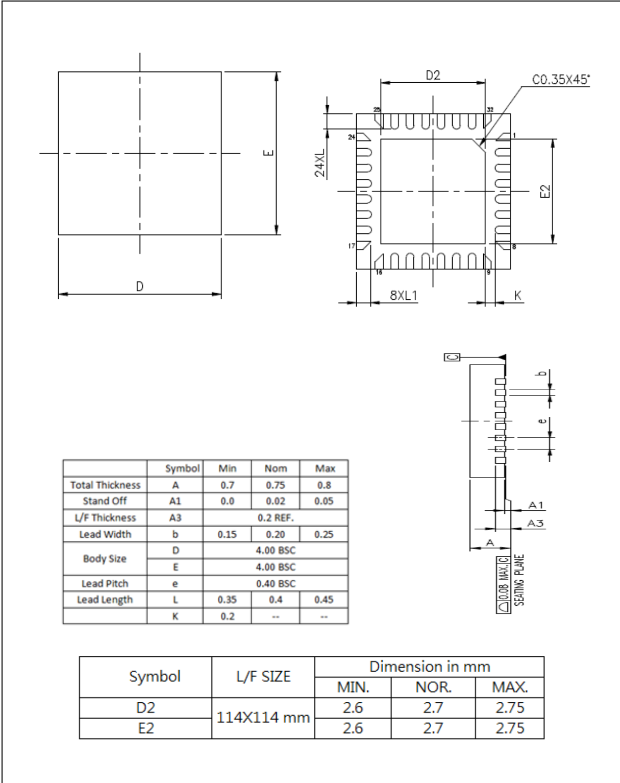
Figure 8.1-1 QFN-33 Package Dimension
