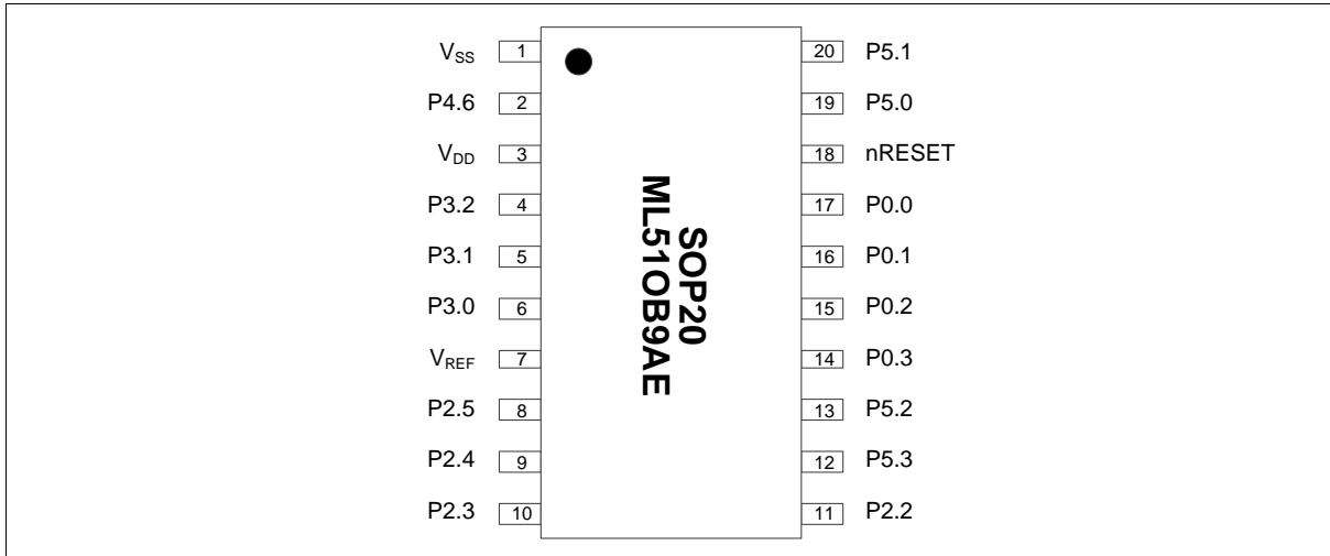
Figure 4.1-6 Pin Assignment of SOP-20 Package
