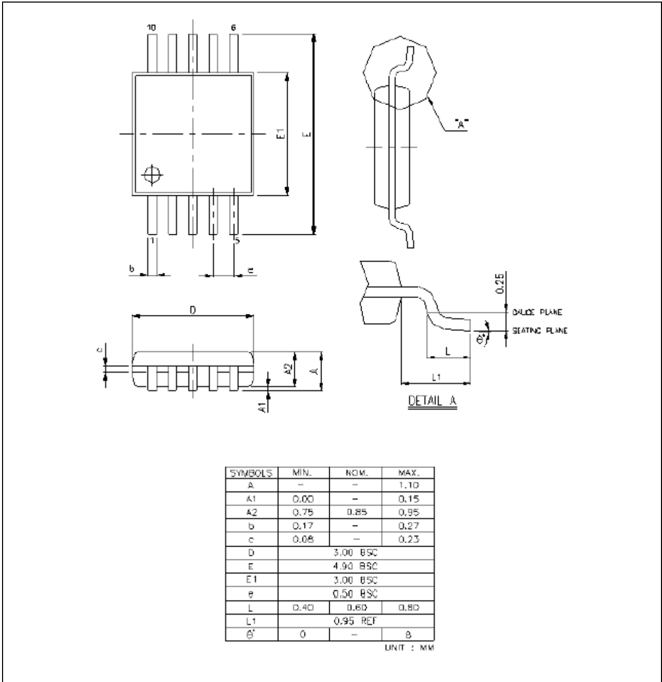
Figure 8.9-1 MSOP-10 Package Dimension
