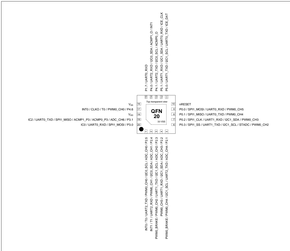
Figure 4.1-16 Multi Function Pin Assignment of QFN-20 Package
