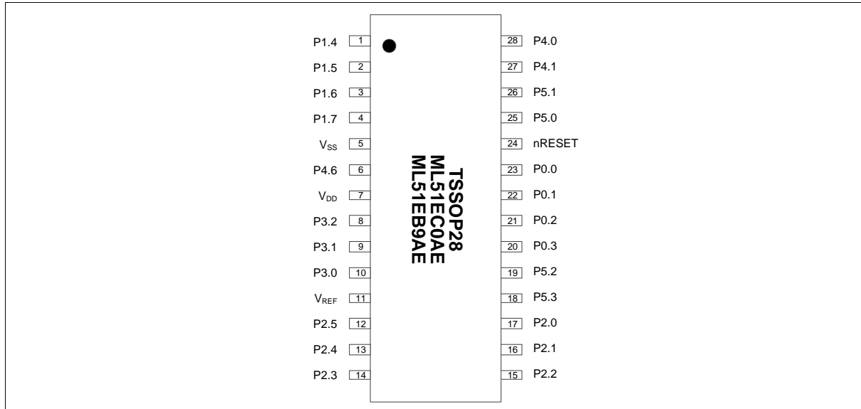
Figure 4.1-3 Pin Assignment of TSSOP-28 Package
