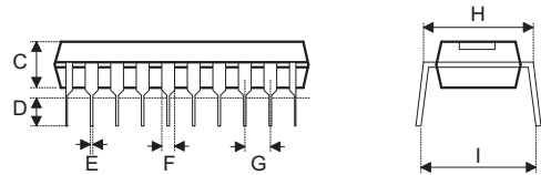
Fig2. 1/2 Lead Packages
