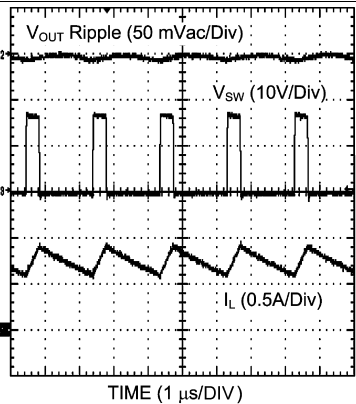
Figure 15. Continuous Mode Operation ( V_{OUT} = 3.3\text{ V} , 2.5\text{ A} Loaded)
