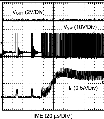
Figure 17. DCM to CCM Transition ( V_{OUT} = 3.3\text{ V} , 0.01\text{ A} - 0.75\text{ A} Load)
