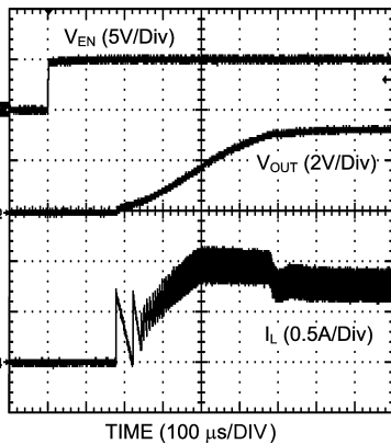
Figure 13. Enable Transient ( V_{OUT} = 3.3\text{ V} , 0.75\text{ A} Loaded)
