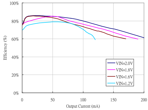
Fig 64. HT7727S Efficiency vs. Output Current
