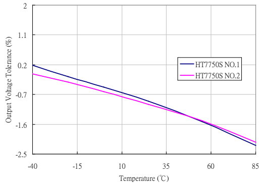
Fig 7. HT7750S Output Voltage Tolerance vs. Temperature
