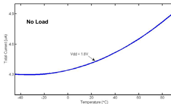
Supply Current over Temperature
