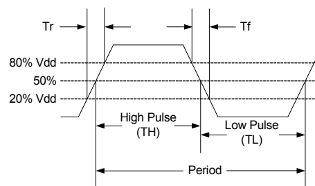
Figure 3. Output Waveform
