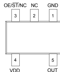
Figure 1. Pin Assignments
