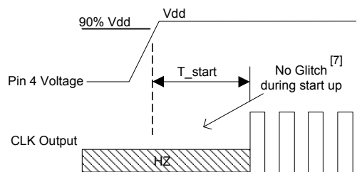
Figure 4. Startup Timing (OE/ST Mode)
