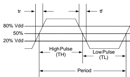
Figure 3. Waveform
