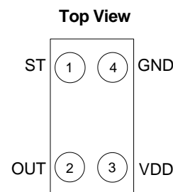
Figure 1. Pin Assignments
