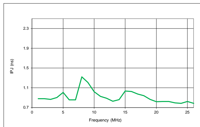
Figure 13. RMS Phase Jitter Random vs Frequency [7]
