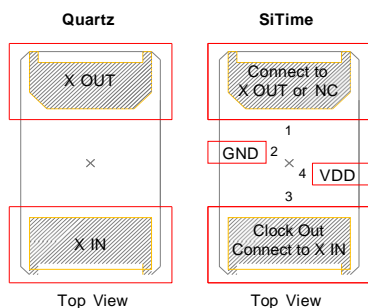
Figure 2. SiT1534 Footprint Compatibility with Quartz XTAL Footprint [5]
