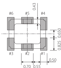
Example of a Terminal Land Pattern
