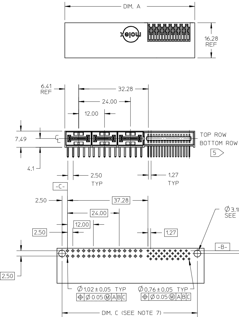
PCB LAYOUT: COMPONENT SIDE THKNESS: SEE CHART
