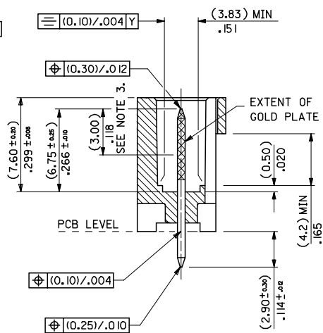
SECTION K-K
