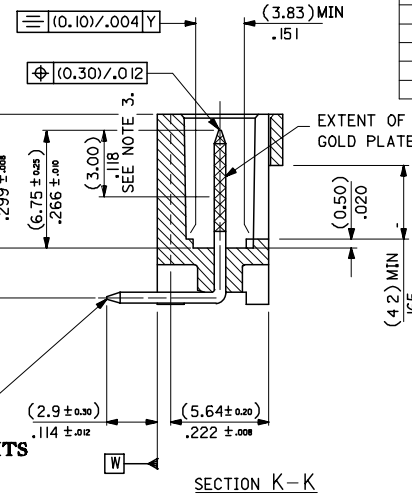
SECTION K-K
