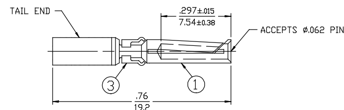
2 PIECE SOCKETS
