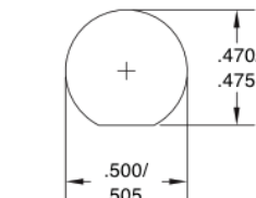
D-Mounting Hole
