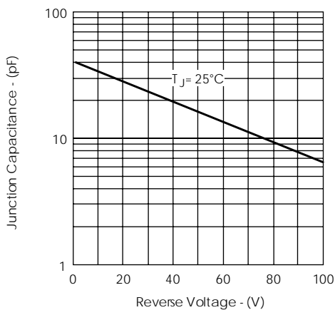
Fig. 3-Typical Junction Capacitance
