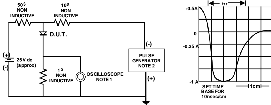
Fig. 1-Reverse Recovery Time Characteristic and Test Circuit Diagram
