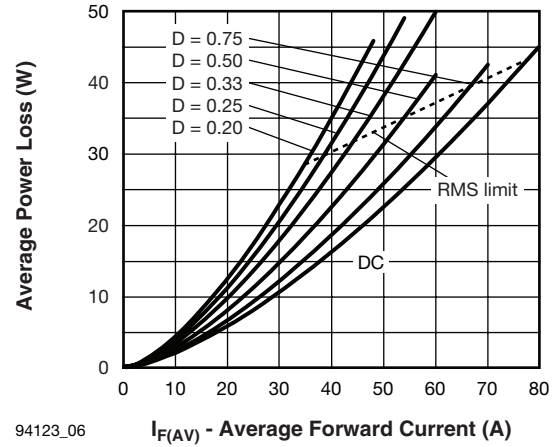
I F(AV) - Average Forward Current (A) Fig. 6 - Forward Power Loss Characteristics (Per Leg)
