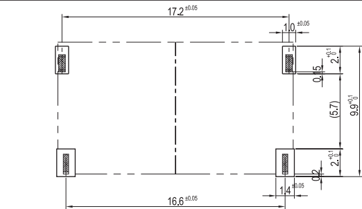
P. C. B. Layout(Connector mounted side)
