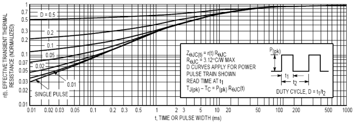
Figure 10. Thermal Response
