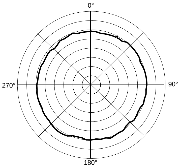
Azimuth 10° Elevation
