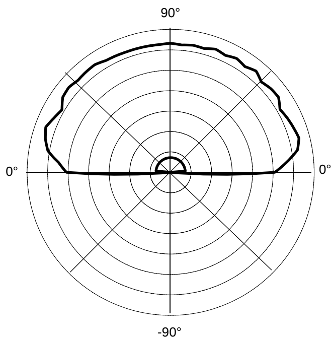
Azimuth 0° Elevation
