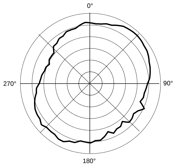
Azimuth 0° Elevation
