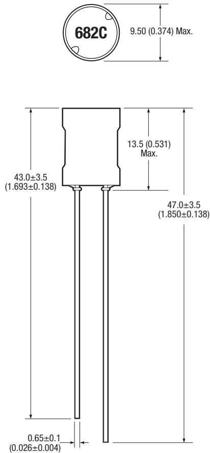
All dimensions in mm (inches). Package weight 2.4g Typ.
