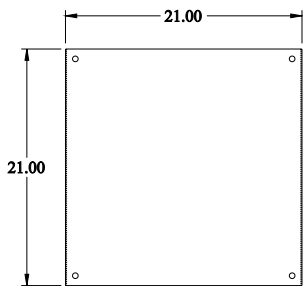
INNER PANEL
