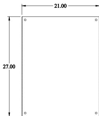
INNER PANEL
