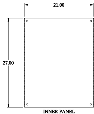
INNER PANEL
