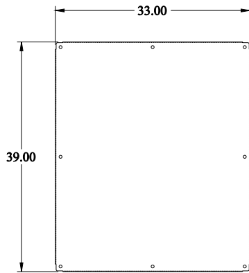
INNER PANEL
