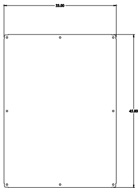
INNER PANEL
