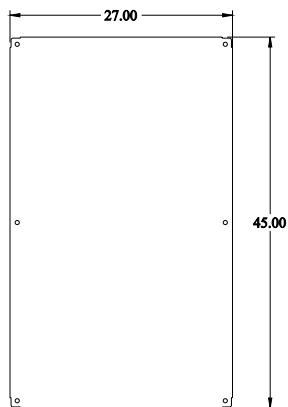
INNER PANEL
