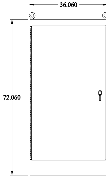
FRONT VIEW
