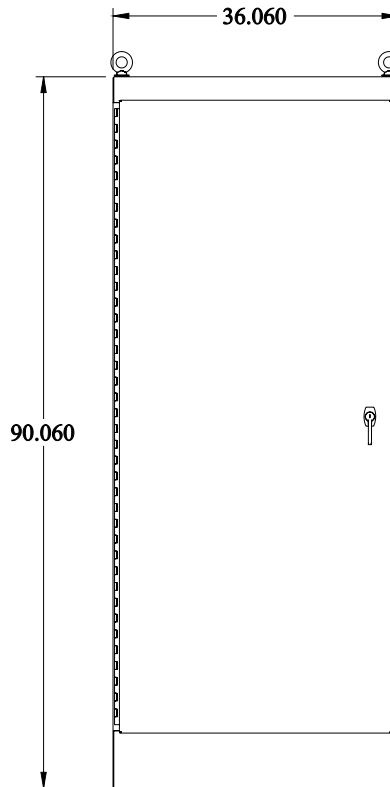
FRONT VIEW
