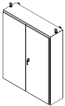
ISOMETRIC VIEW
