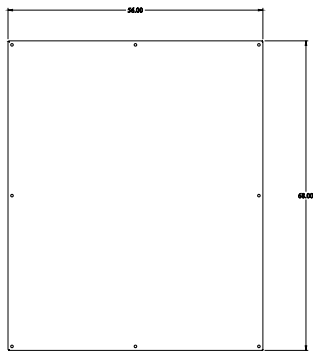
INNER PANEL
