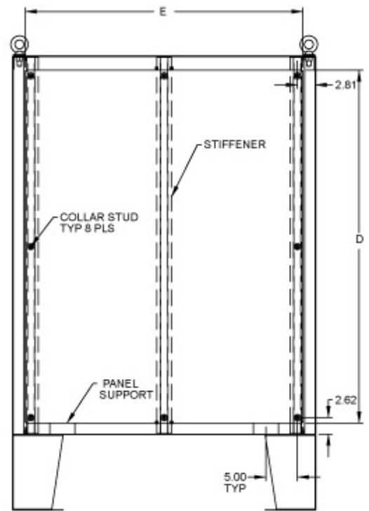
SECTION Y-Y
