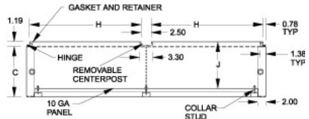
Section X-X
