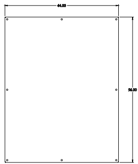
INNER PANEL
