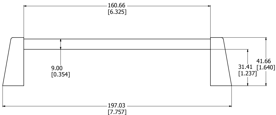
SIDE VIEW
