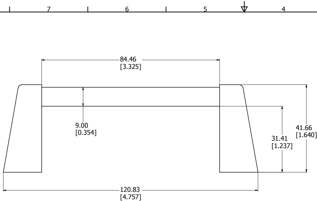
SIDE VIEW
