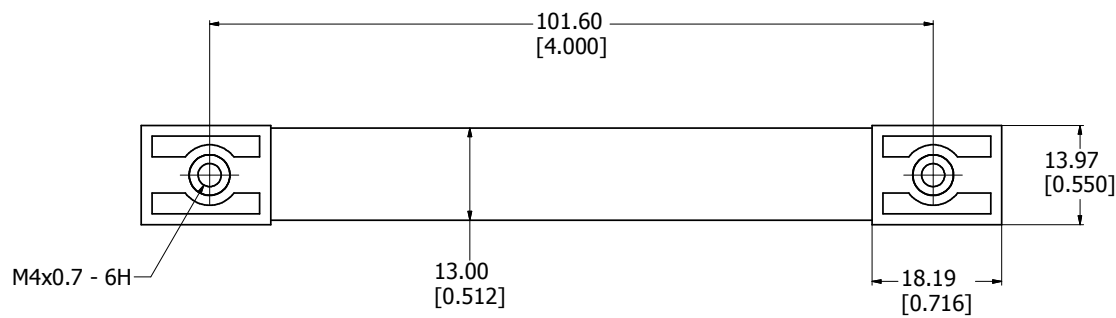
BOTTOM VIEW
