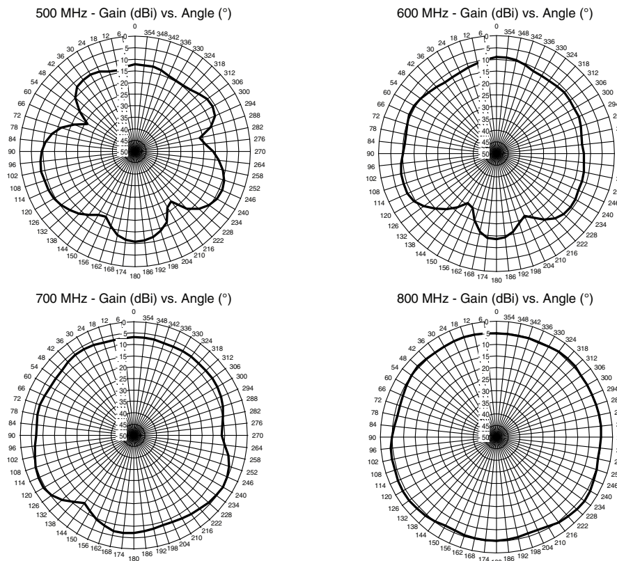
Fig. 5 - Measured Radiation Pattern
