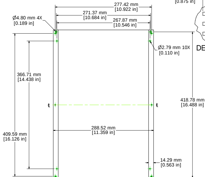
TOP PANEL - BOTTOM VIEW
