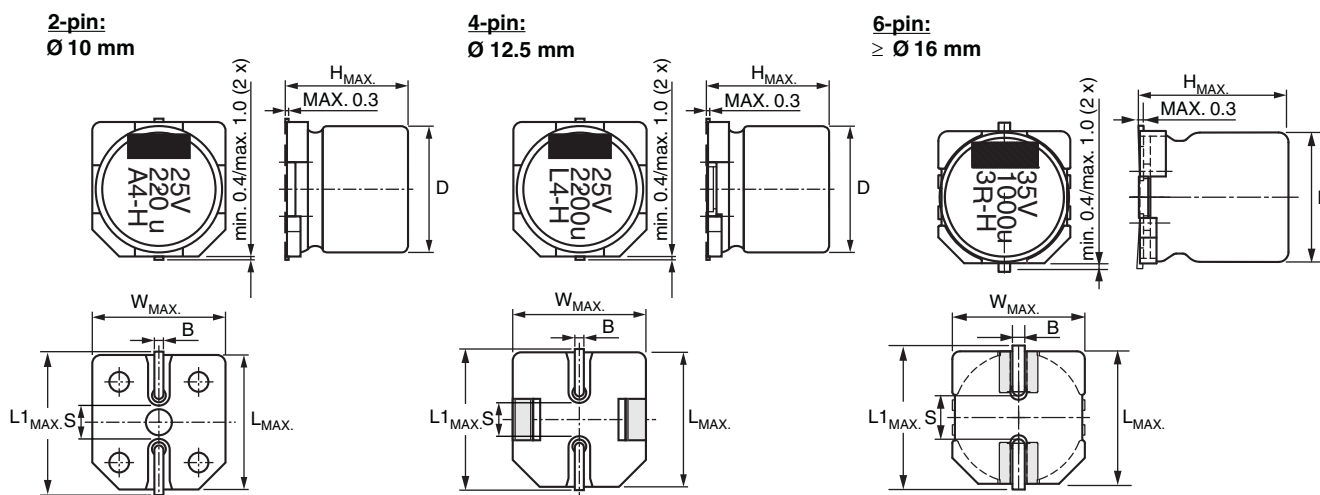
Fig. 2 - Dimensional outline
