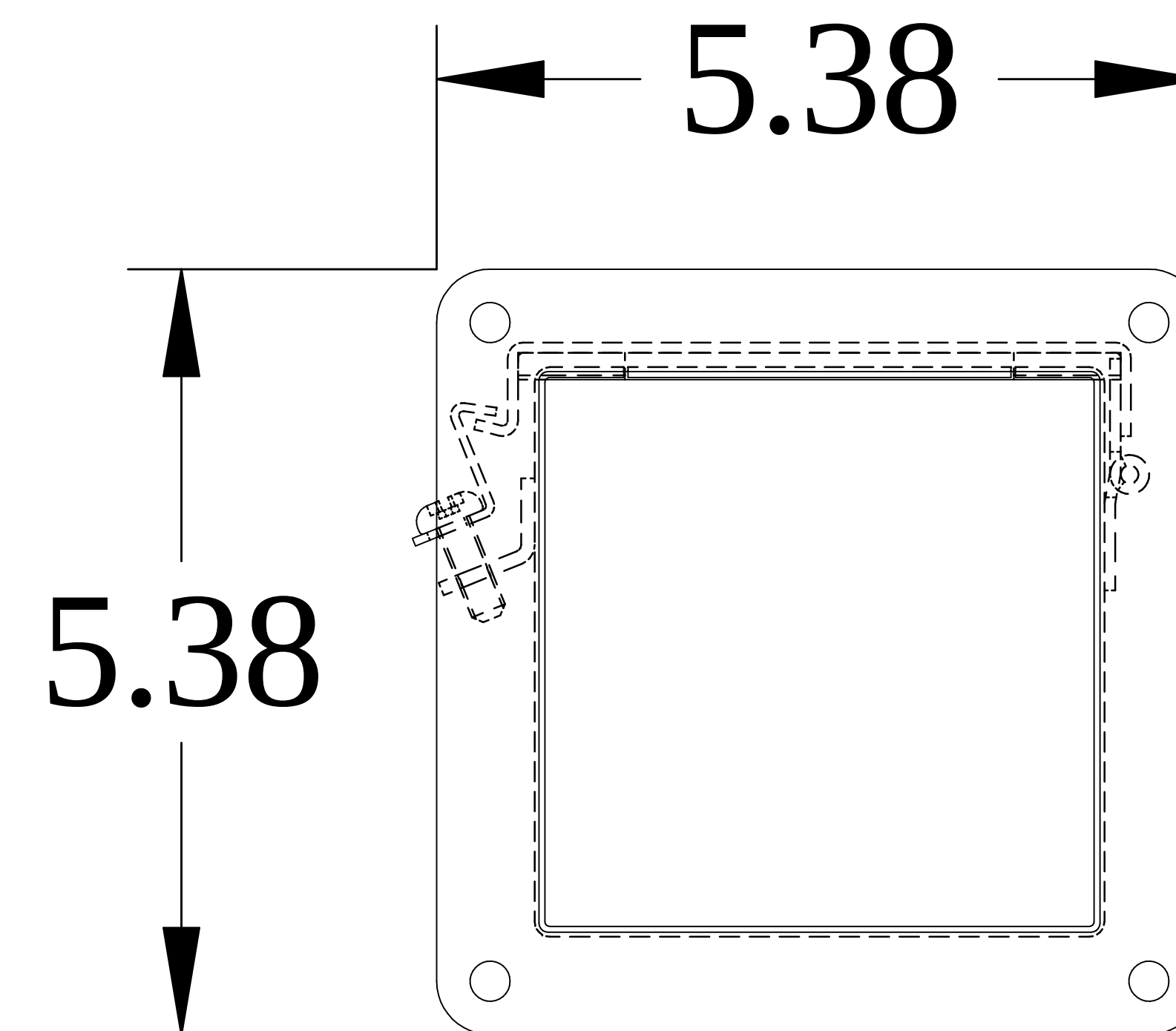
END VIEW
