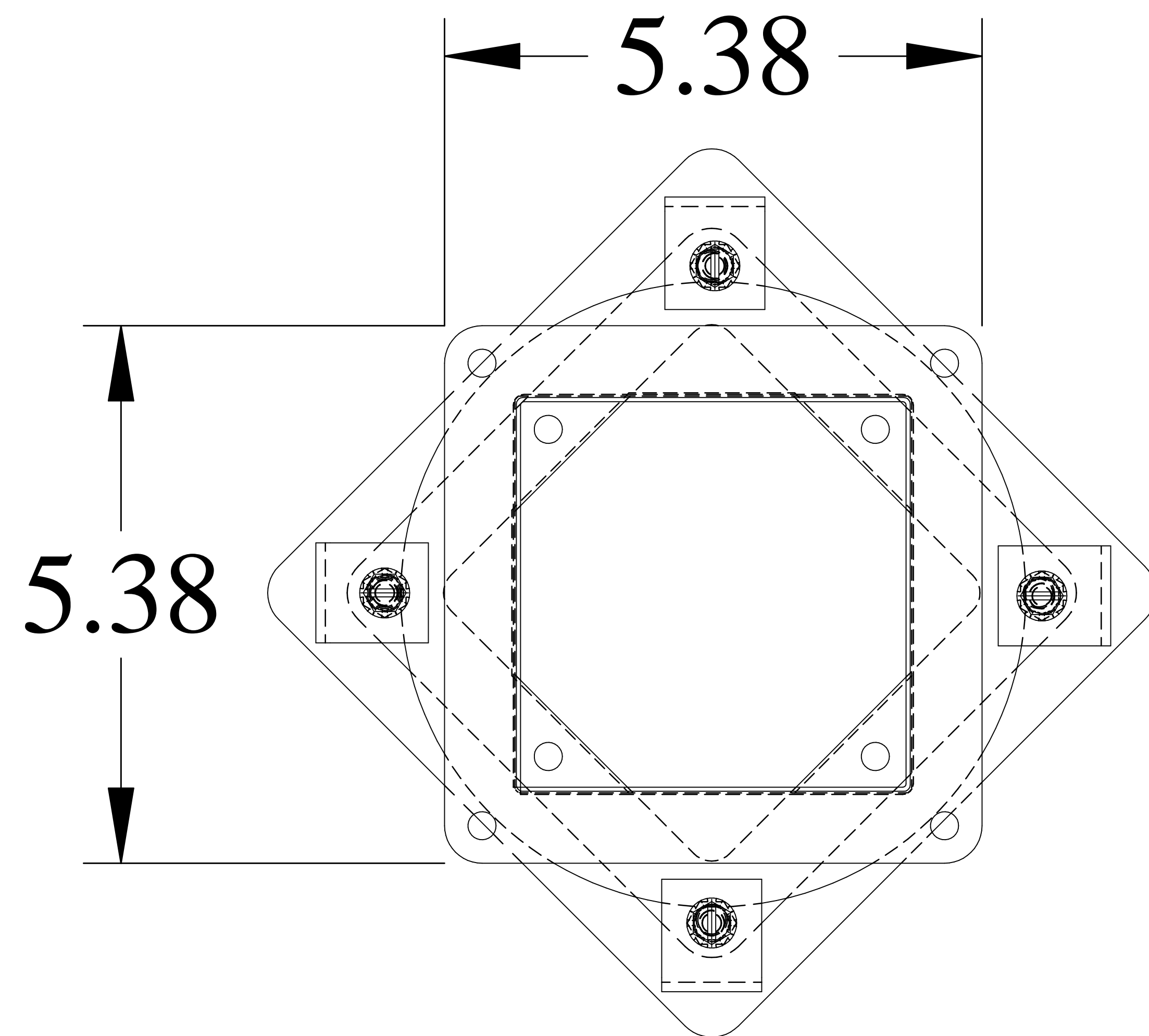
FRONT VIEW
