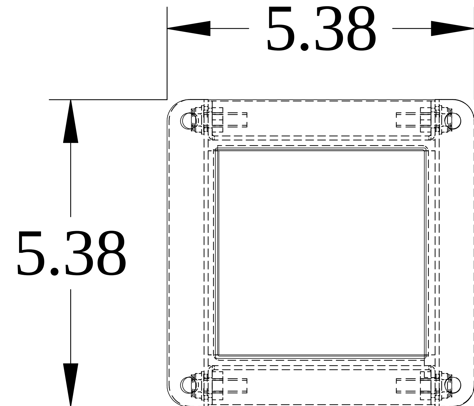
END VIEW
