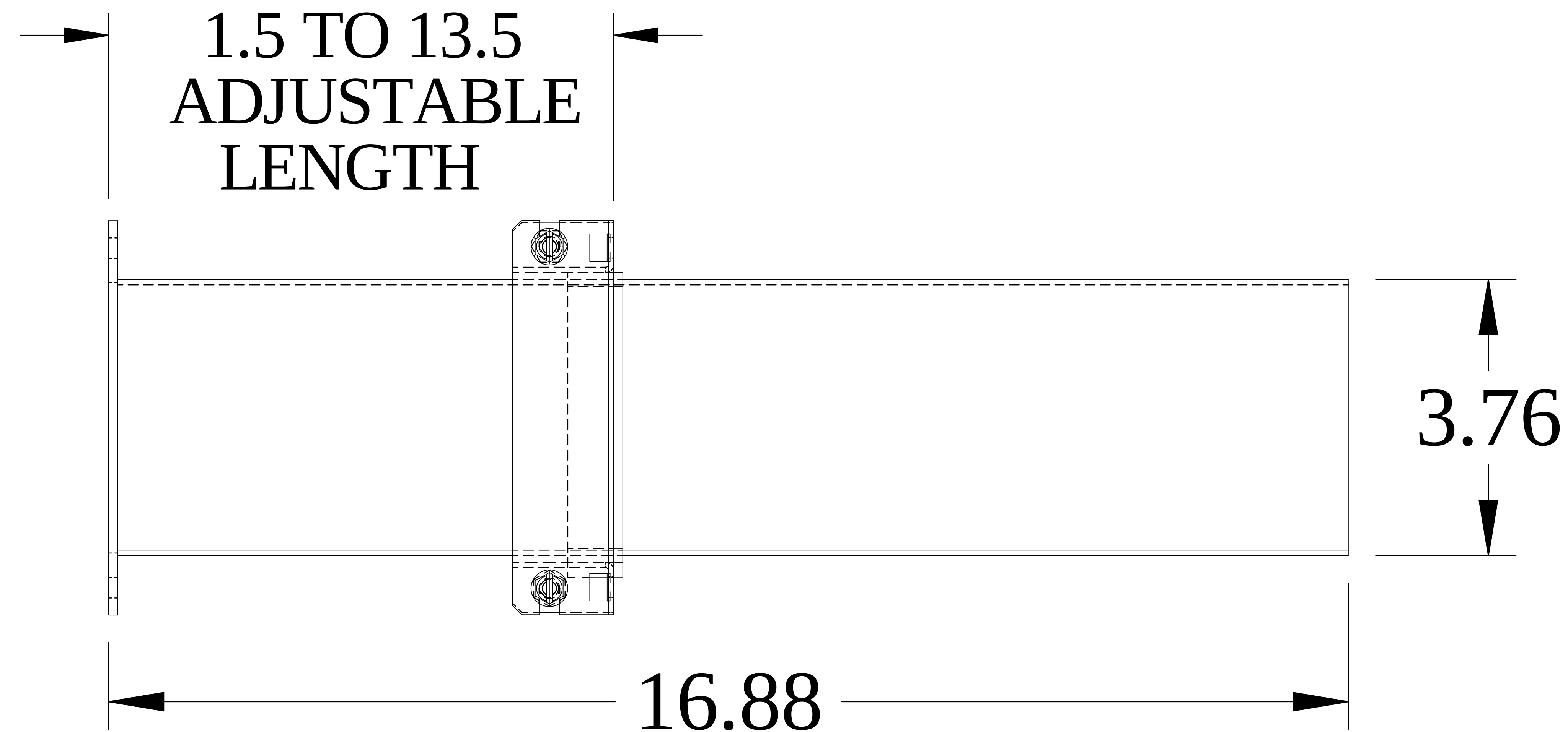
SIDE VIEW
