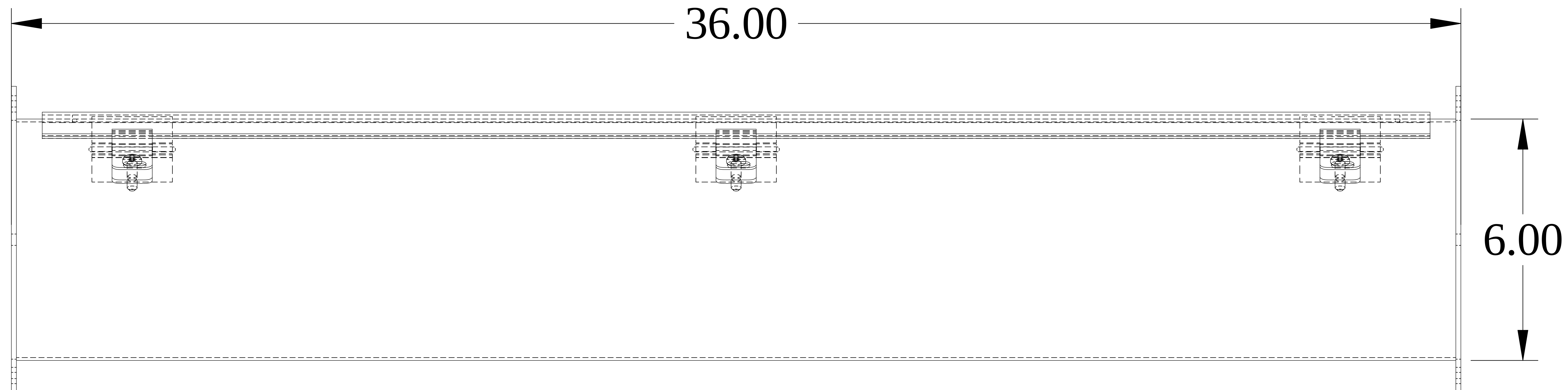
SIDE VIEW
