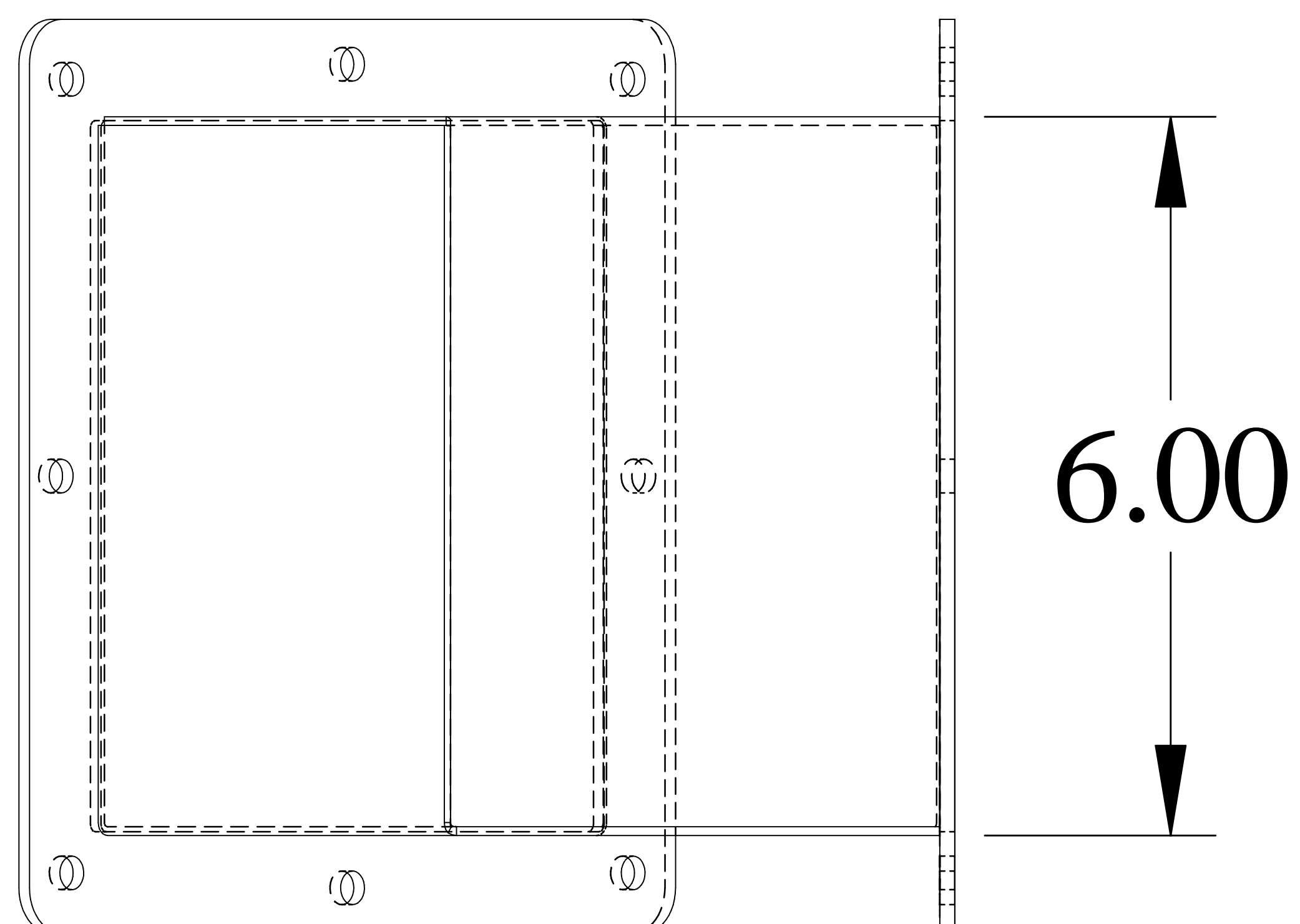
FRONT VIEW
