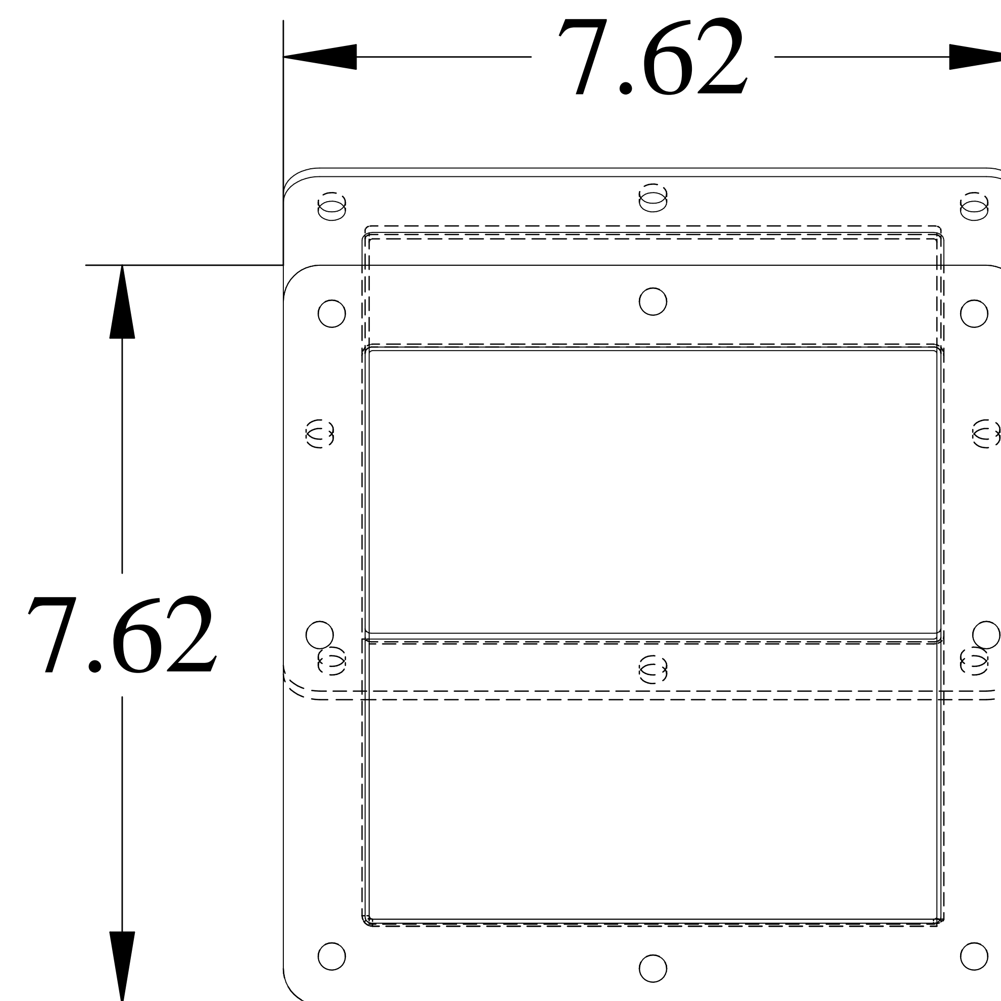
END VIEW
