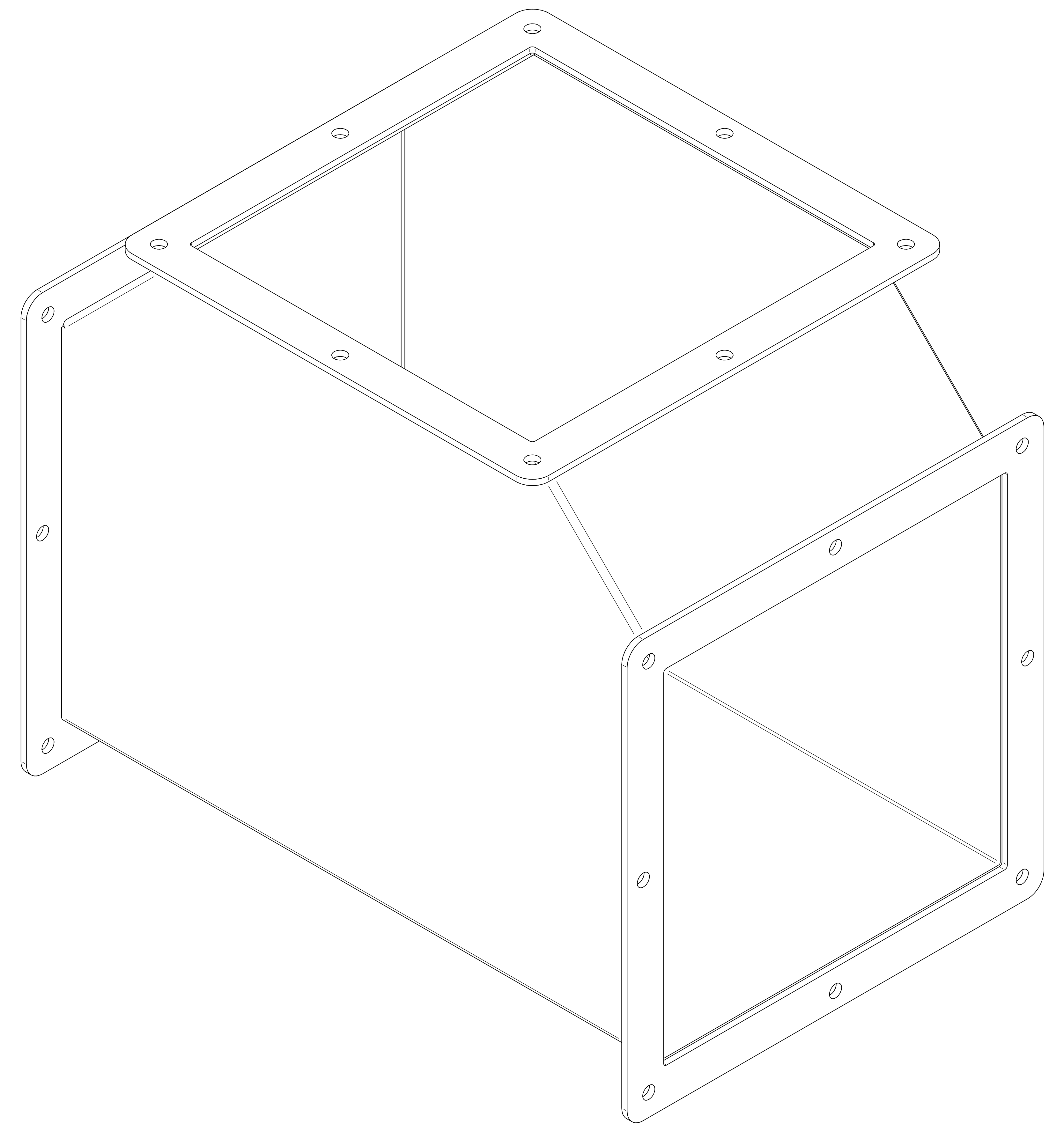
ISOMETRIC VIEW
