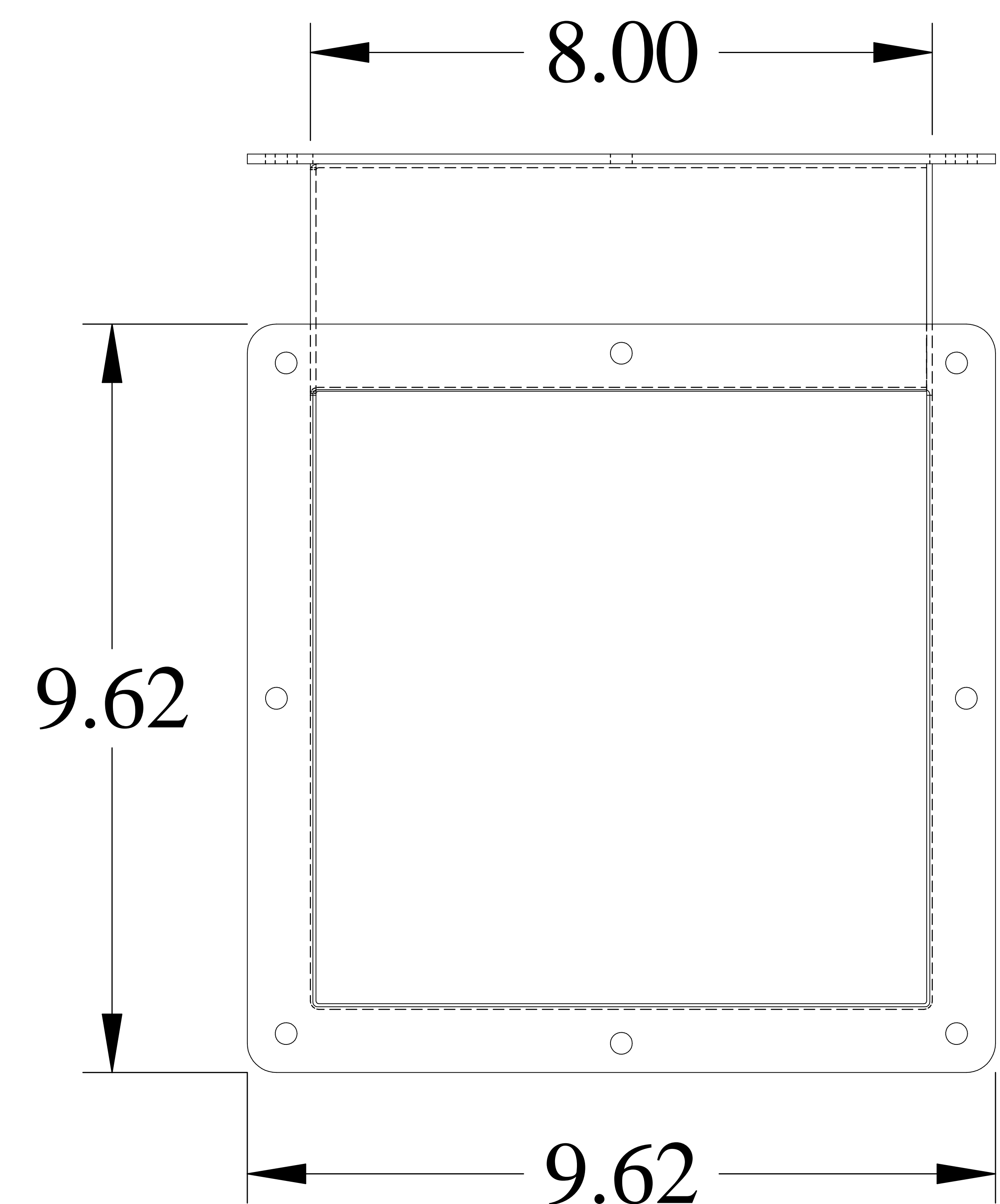
SIDE VIEW
