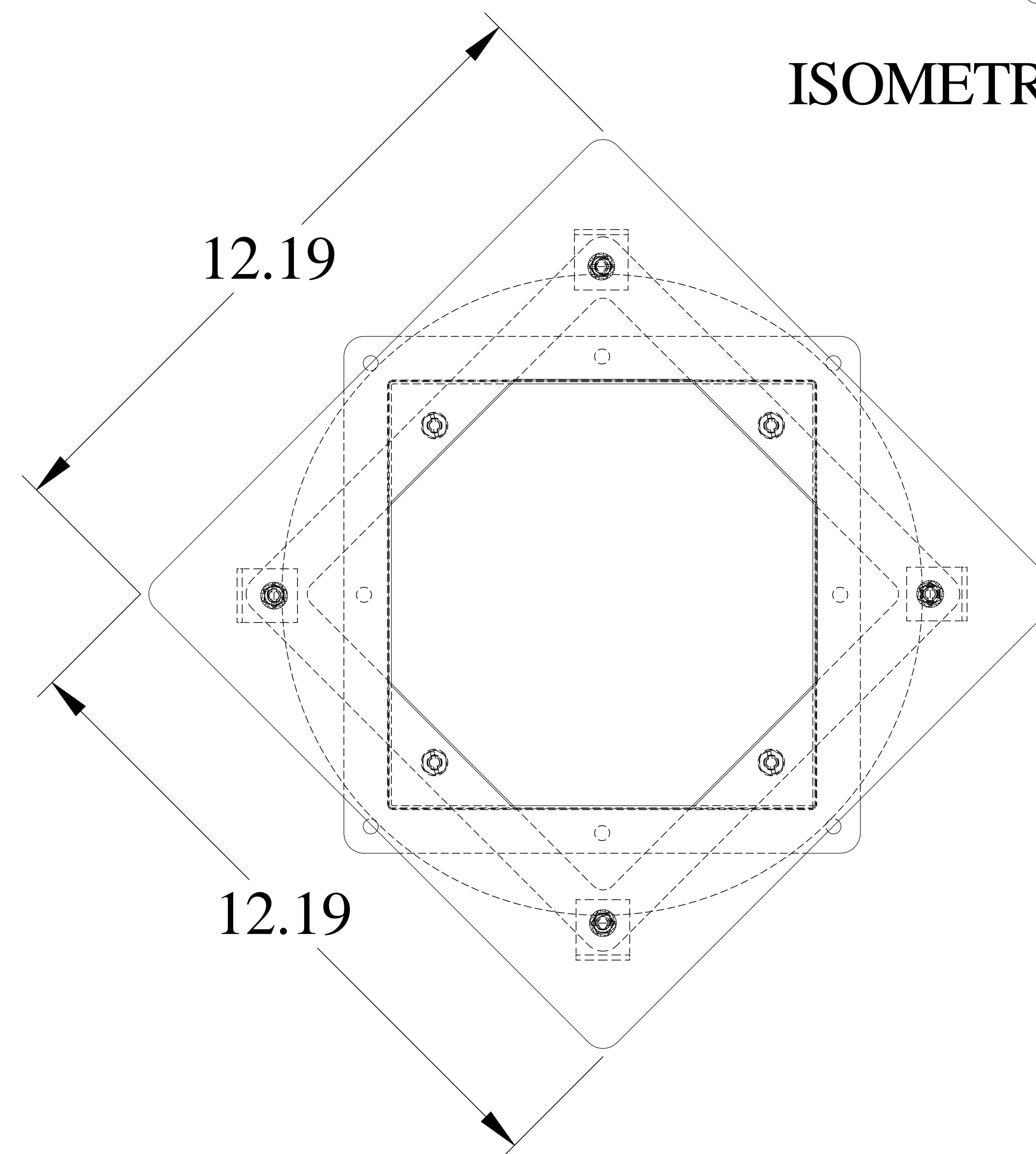
BACK VIEW
