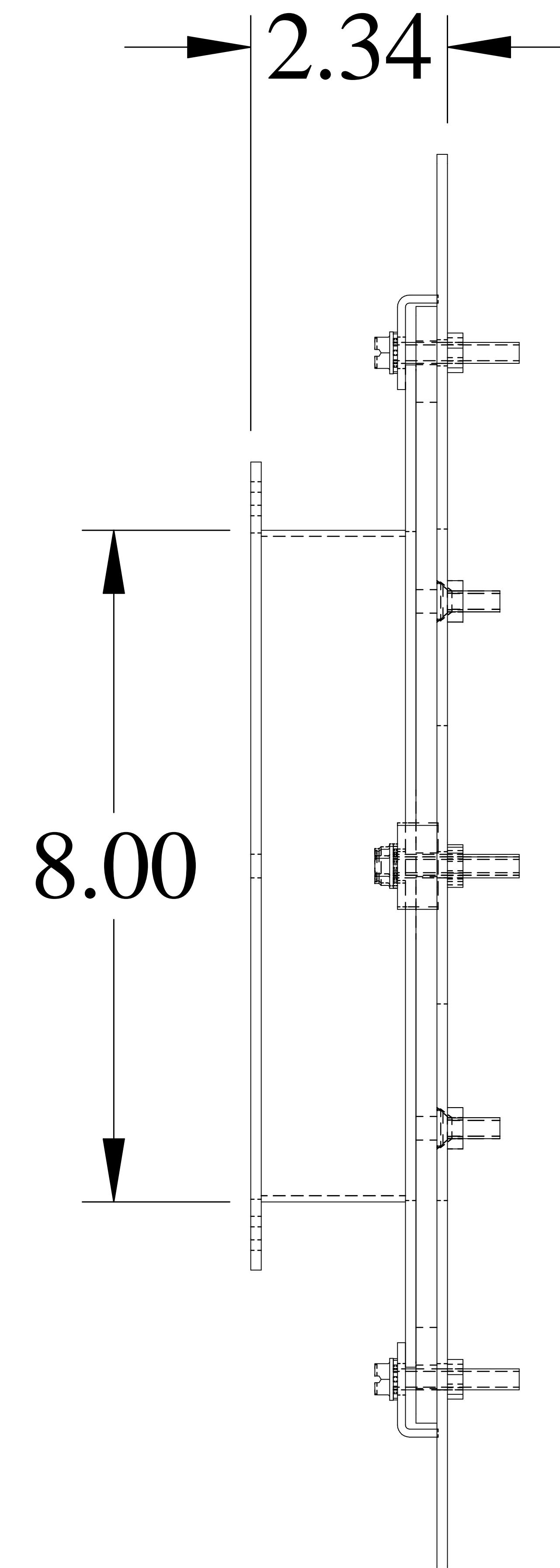
SIDE VIEW
